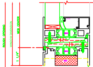
241 SILL 325 CASEMENT OUT BUTT HINGES
