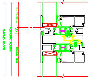
541 MEETING RAIL 325 FIXED \ CASEMENT OUT BUTT HINGES
