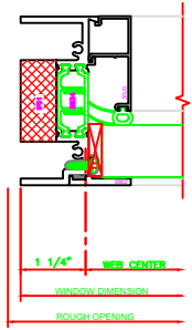
403 JAMB 325 PROJECT OUT \ FIXED
