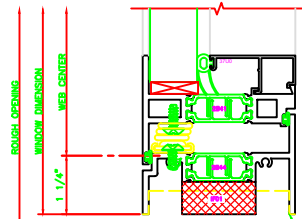
240 SILL 325 CASEMENT OUT 4-BAR ARMS
